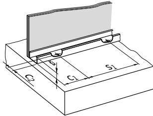
Fixed track fastening
