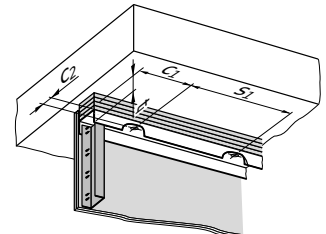
Deflection head track fastening with gypsum strips (optional with sealant)
