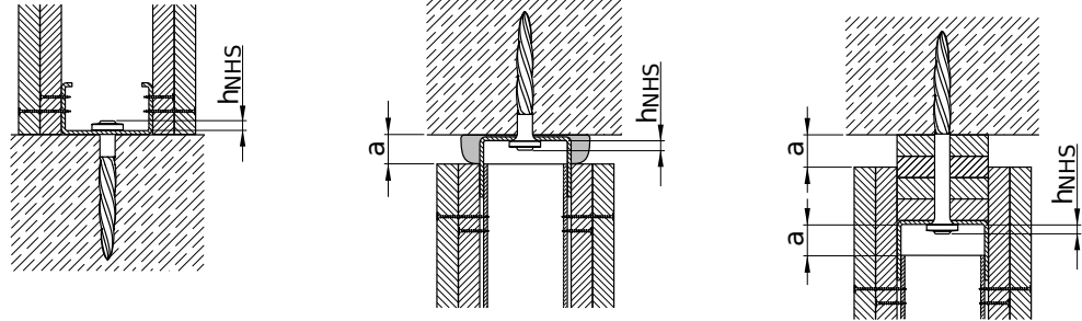
Fixed track fastening Deflection head track fastening (optional with sealant) Deflection head fastening with gypsum strips (optional with sealant)
